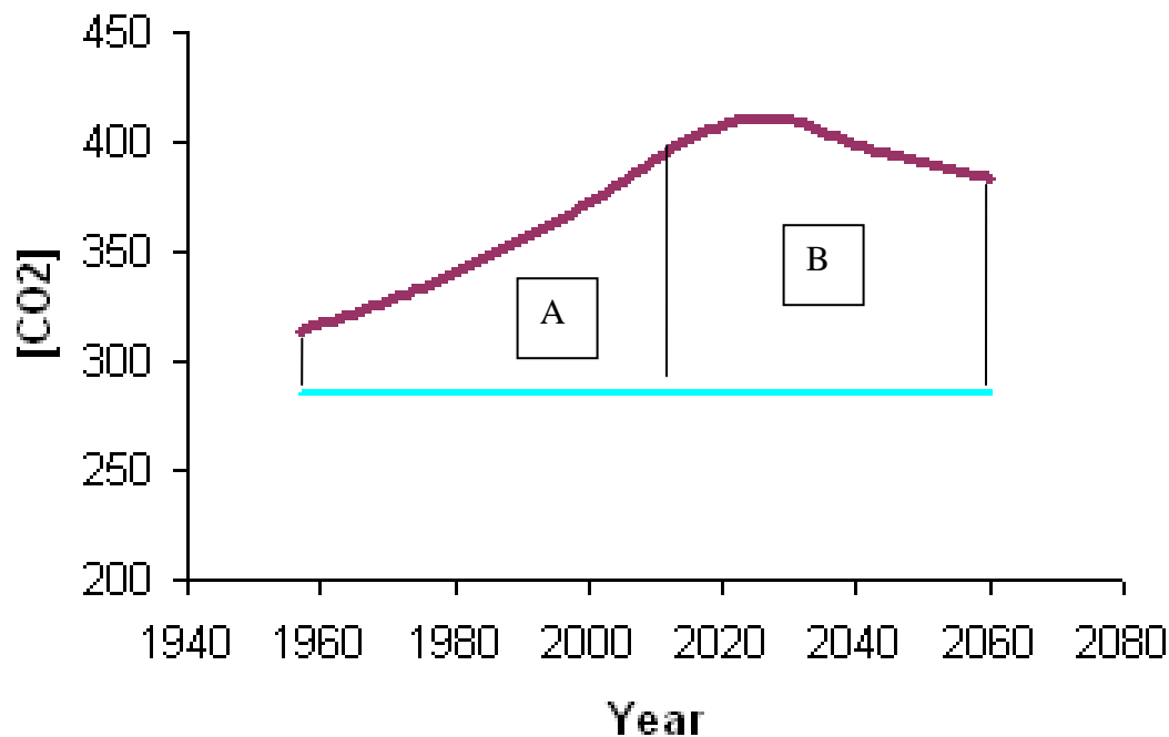
Figure 1 Excess CO 2 over the preindustrial level for the last 50 years and for the next 50 assuming emissions fall to zero by 2035 and remain zero thereafter
